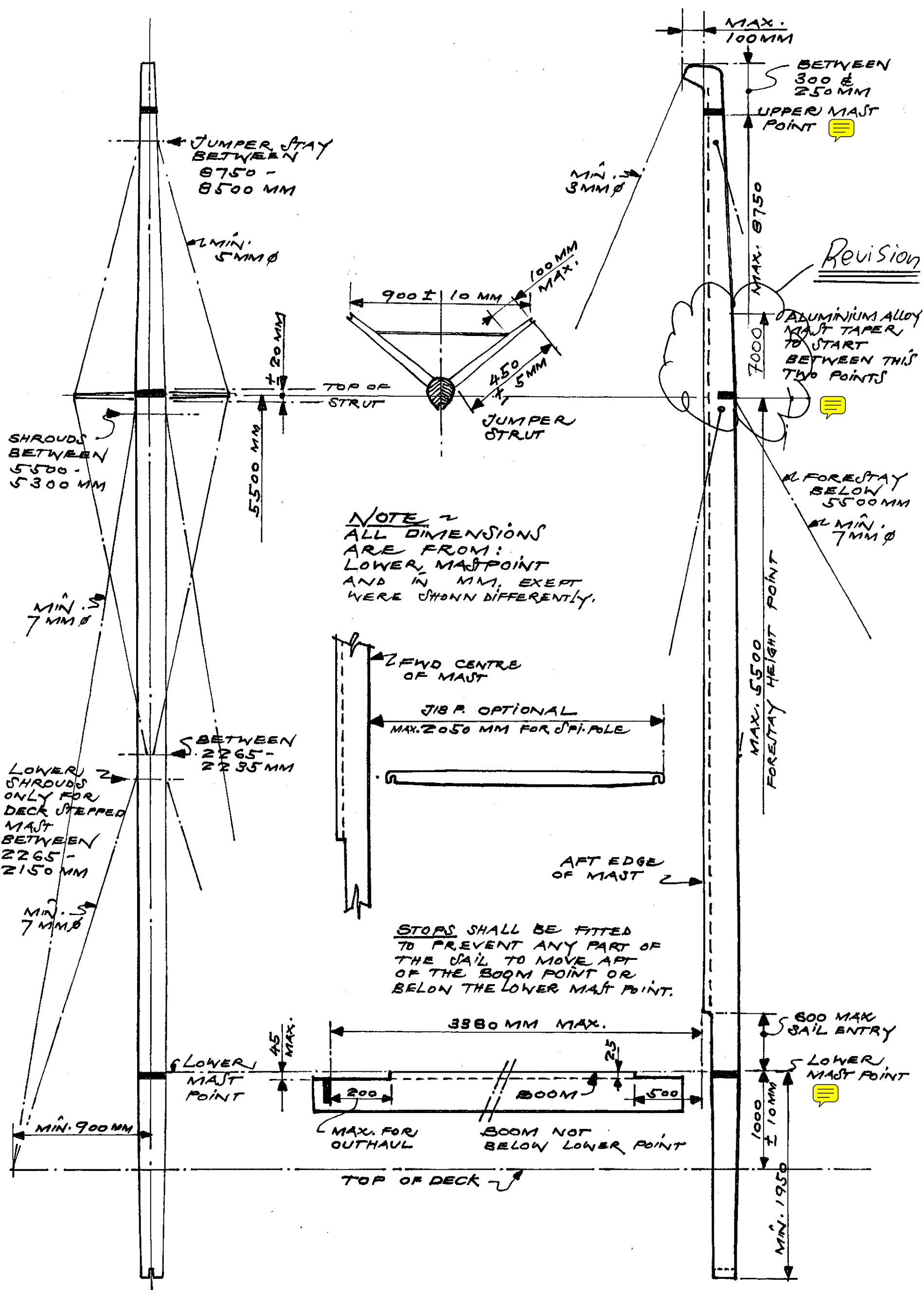
NORDIC FOLKBOAT SPAR & RIG DIAGRAM NO SCALE 3.4.03 G.O. AHLER DRG. No 11
